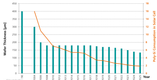
c-Si Solar Cell Development Wafer Thickness [ \mu\text{m} ] & Silicon Usage [g/Wp]
