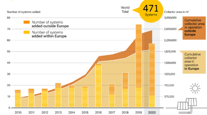
Solar District Heating, Global Annual Additions and Total Area in Operation 2010-2020
