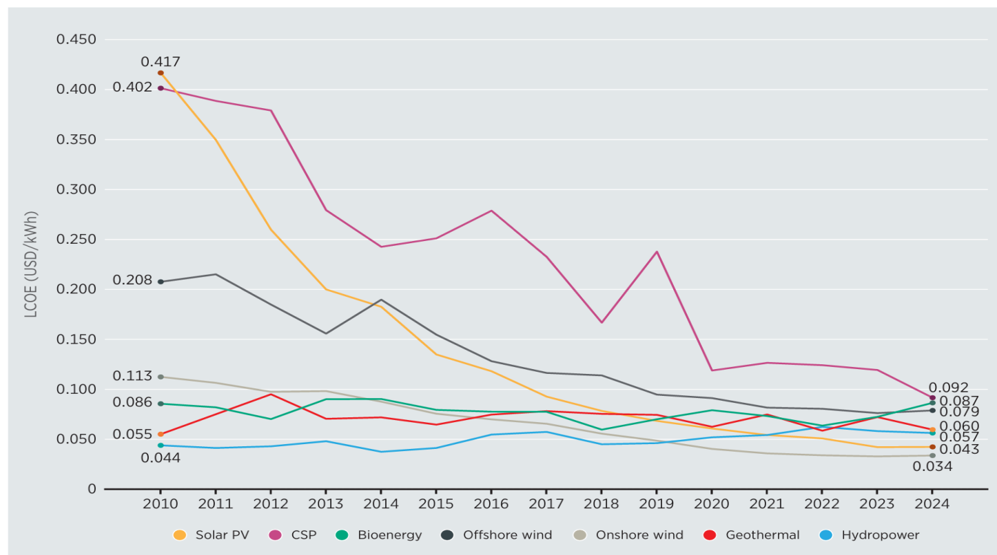
Figure S1 Renewable energy LCOE decline, 2010-2024
