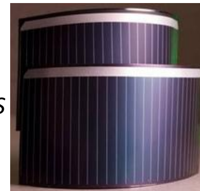
Cl(G)S
