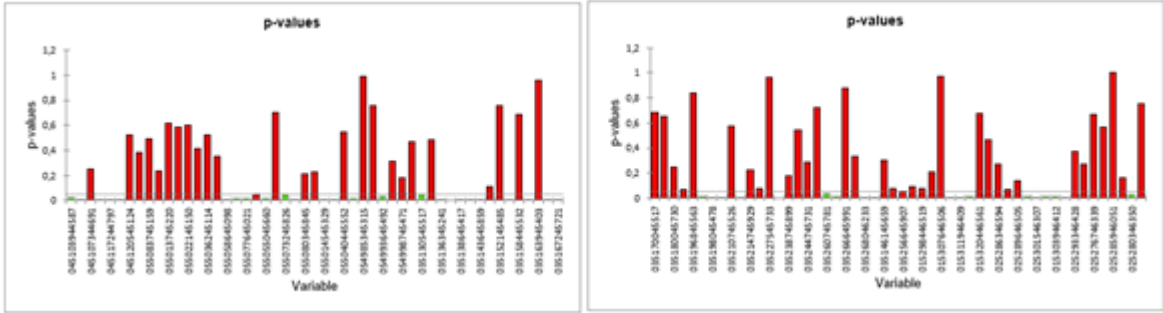
Figure 3.2.3 Results of Mann- Kendall trend test
