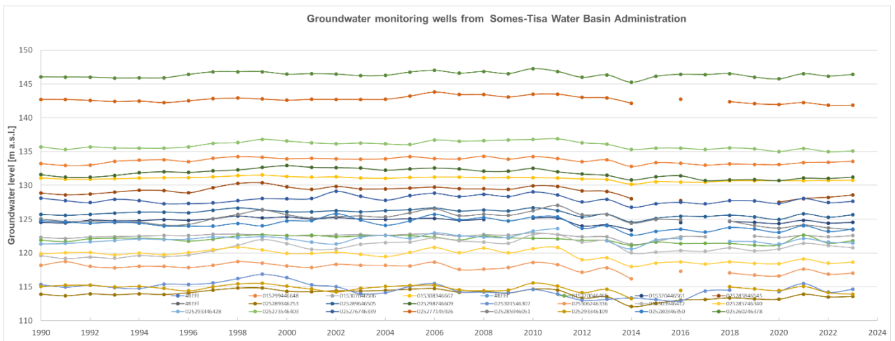
Figure 3.2.1.d) Groundwater change of obs. wells in the Somes-Tisa River basin (1990-2022)
