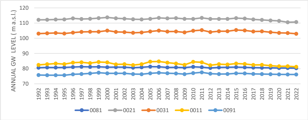
Figure 3.5.1 Groundwater change of obs. Wells in Serbia (1990-2022)
