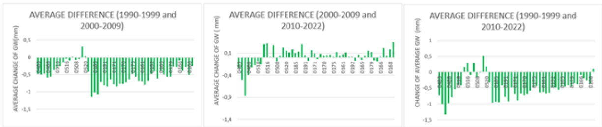
Figure 3.3.6 Differences in average GW levels between decades- the Sava river basin
