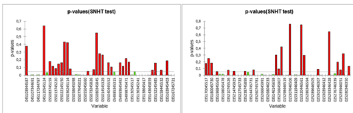
Figure 3.2.2 Results of SNHT for 98 obs. wells in Romania
