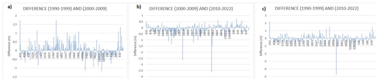
Figure 3.6.4 Differences in average GW levels between decades - Hungary
