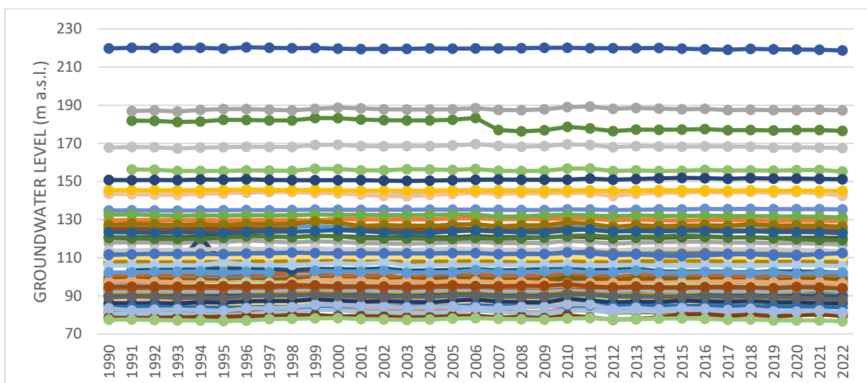
Figure 3.6.1.c) Groundwater change of 65 obs. wells in Hungary (1990-2022)
