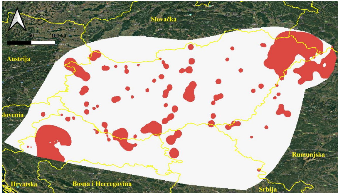
Figure 4.1.1 Critical spots ( Map 10)
