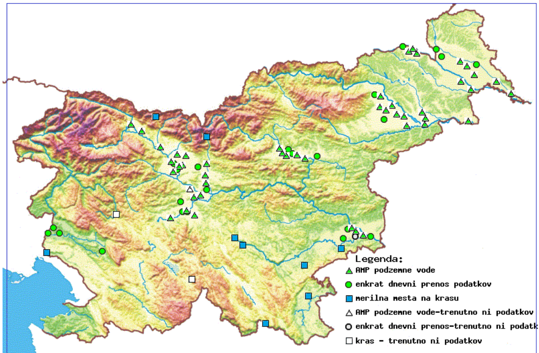
Figure 2.3.1 The network of groundwater wells in Slovenia (green triangle: automatic measuring station; green circle: daily measurement; blue square: karst measuring station; white icons: currently no data available)
