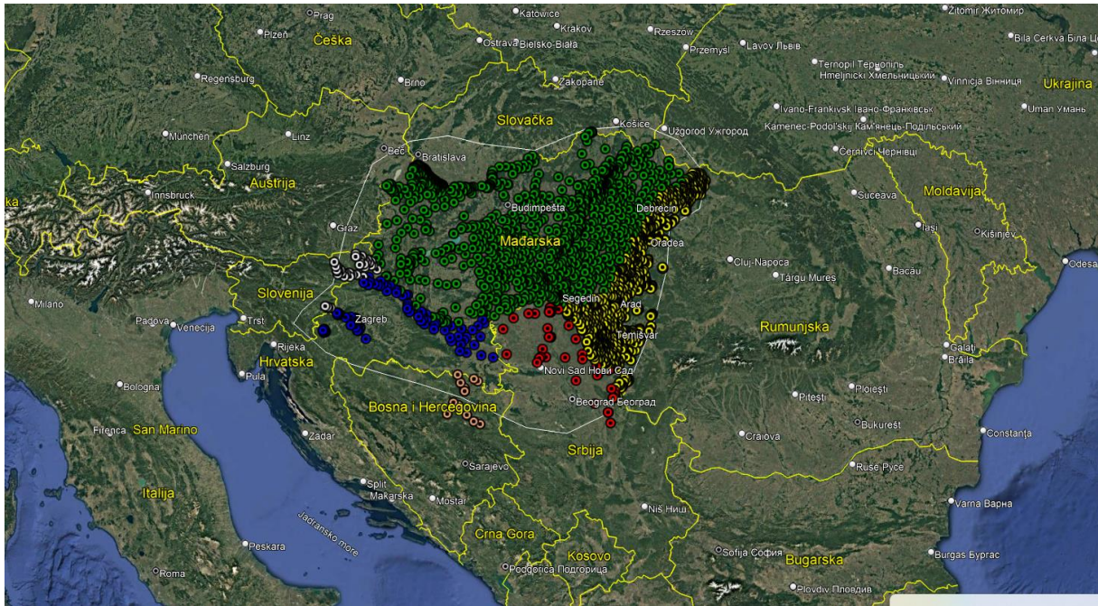
Figure 2.7.1 Presentation of complete GW observation network ( Map 1)
