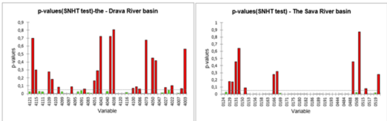
Figure 3.3.3 Results of SNHT for 98 obs. wells in Croatia- the Drava and the Sava River basins
