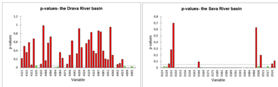
Figure 3.3.4 Results of Mann- Kendall trend test
