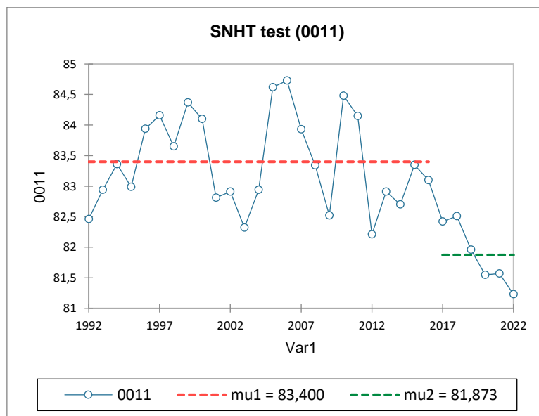
Figure 3.5.3 Results of SNHT for one specific obs. wells in Serbia
