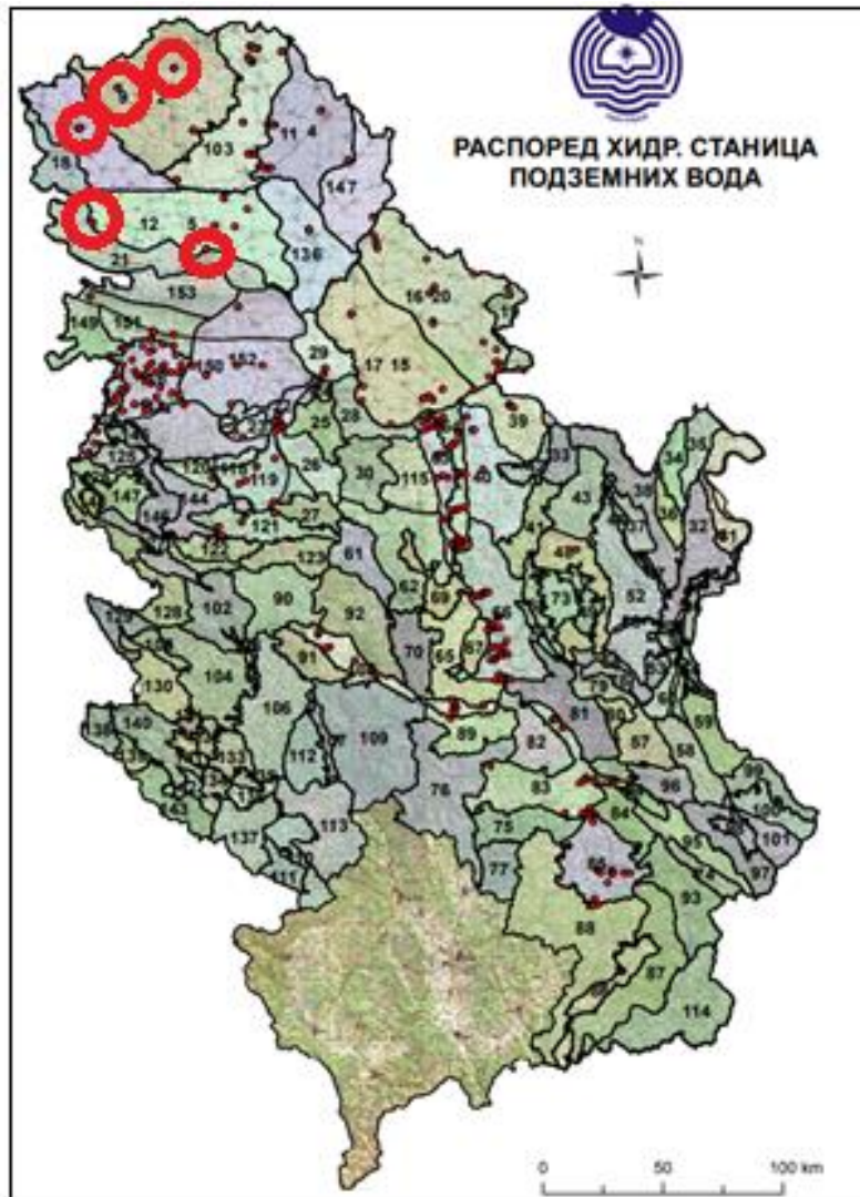
Figure 2.4.1 The network of groundwater wells identified by RHMZ in Serbia in 2023 with designated piesometers included in project area https://www.hidmet.gov.rs/data/hidro_pod_godisnjaci/PODZEMNE%20VODE%202023.pdf
