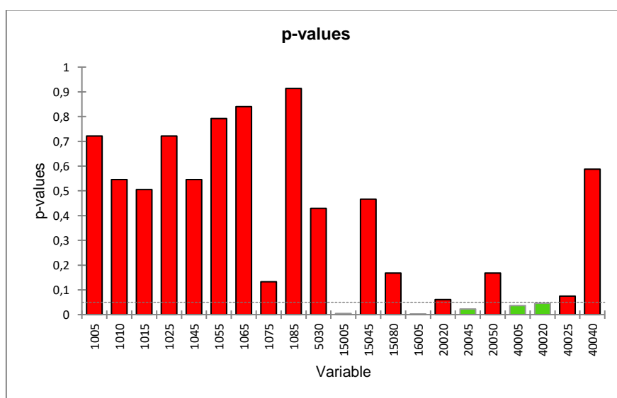
Figure 3.4.3 Results of Mann- Kendall trend test
