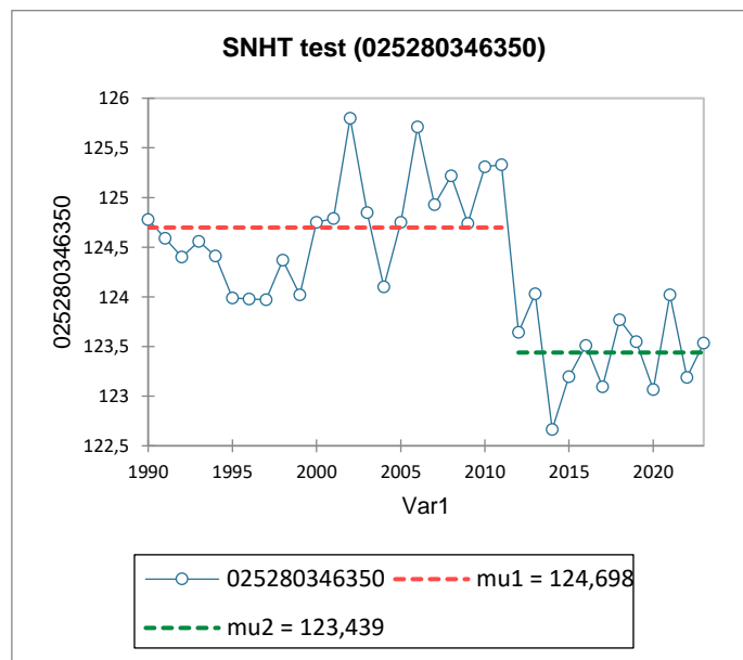
Figure 4.1.2 Example of GW lowering in the Somes-Tisa river basin in Romania
