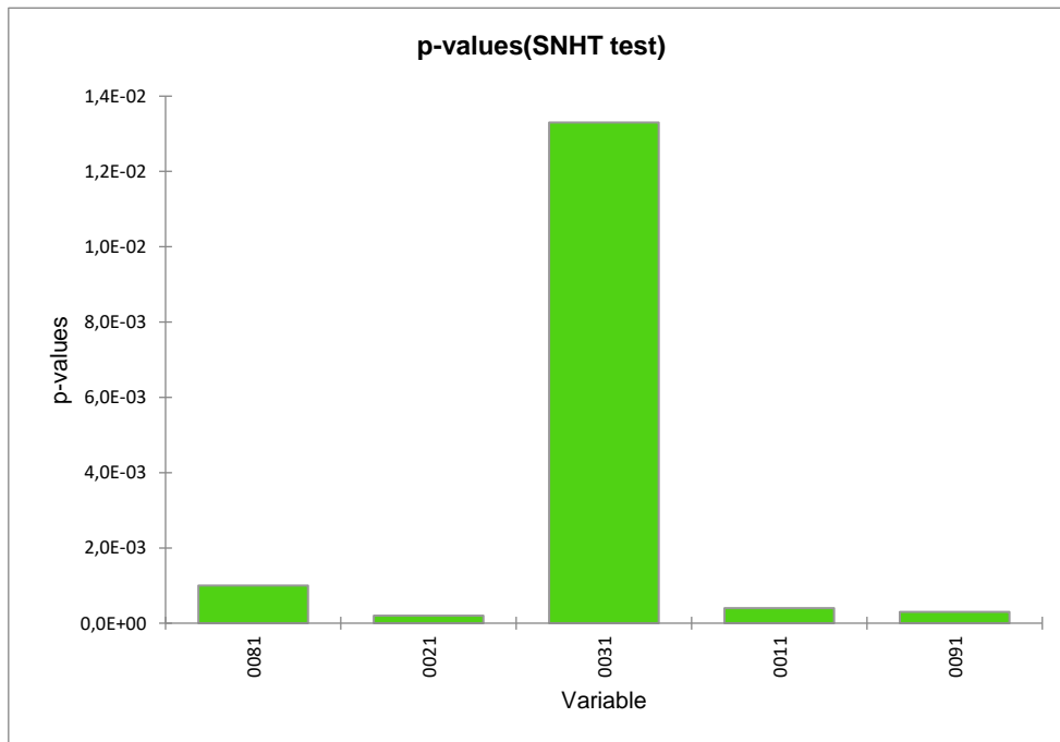
Figure 3.5.2 Results of SNHT for 5 obs. wells in Serbia
