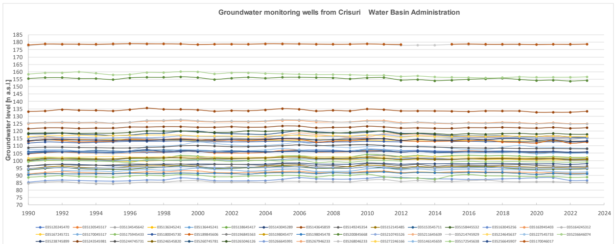
Figure 3.2.1.c) Groundwater change of obs. wells in the Crisuri water basin (1990-2022)
