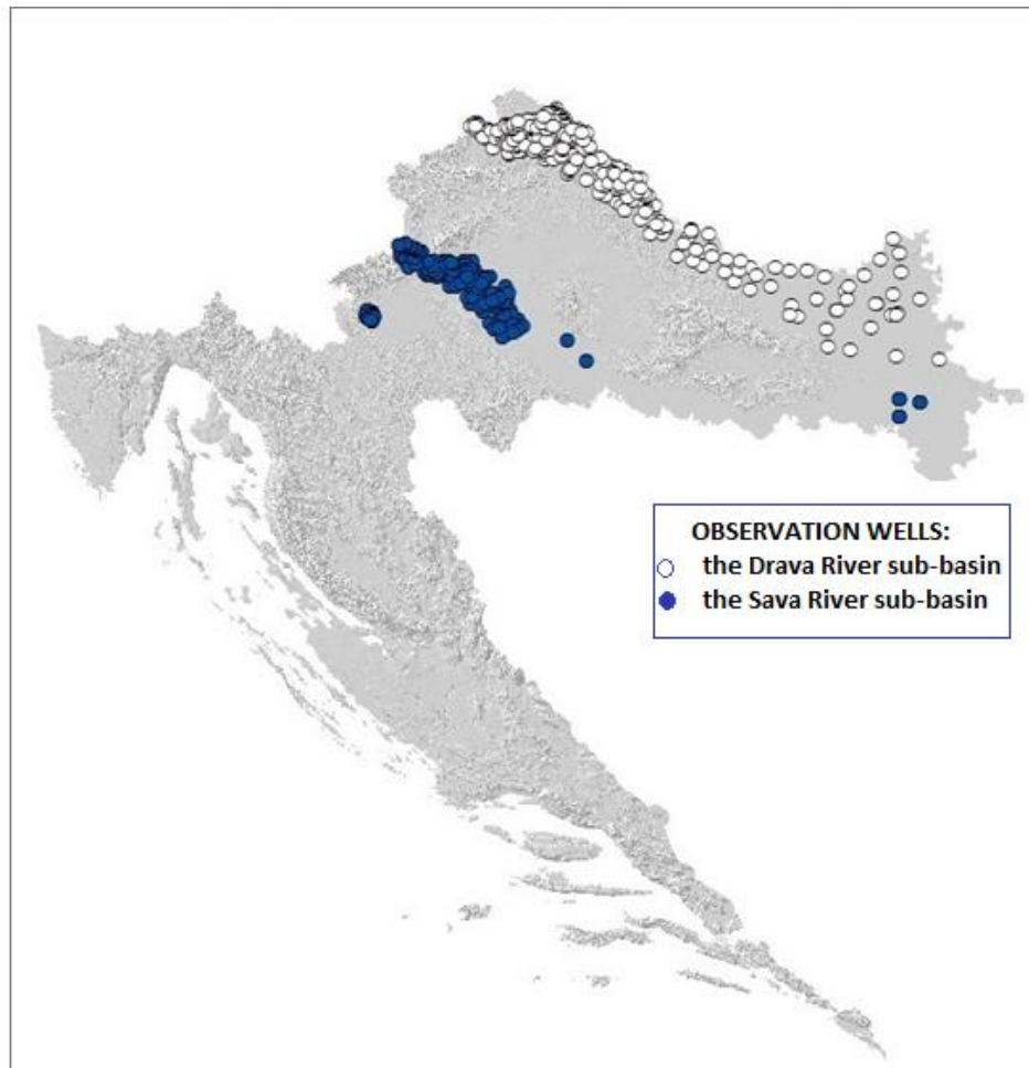
Figure 2.2.1 The network of groundwater wells identified by DHMZ in Croatia ( https://meteo.hr/infrastruktura.php?section=mreze_postaja&param=hm&el=podzemne_hm )
