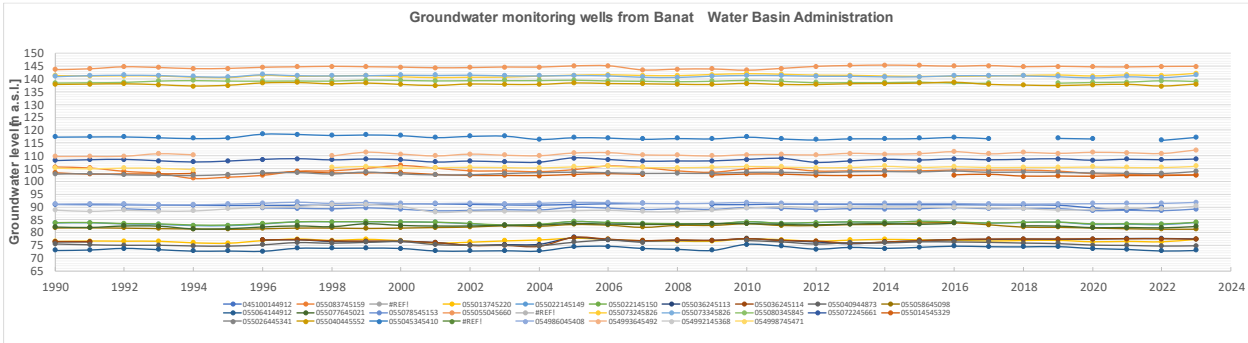
Figure 3.2.1.a) Groundwater change of obs. wells in the Banat water basin (1990-2022)
