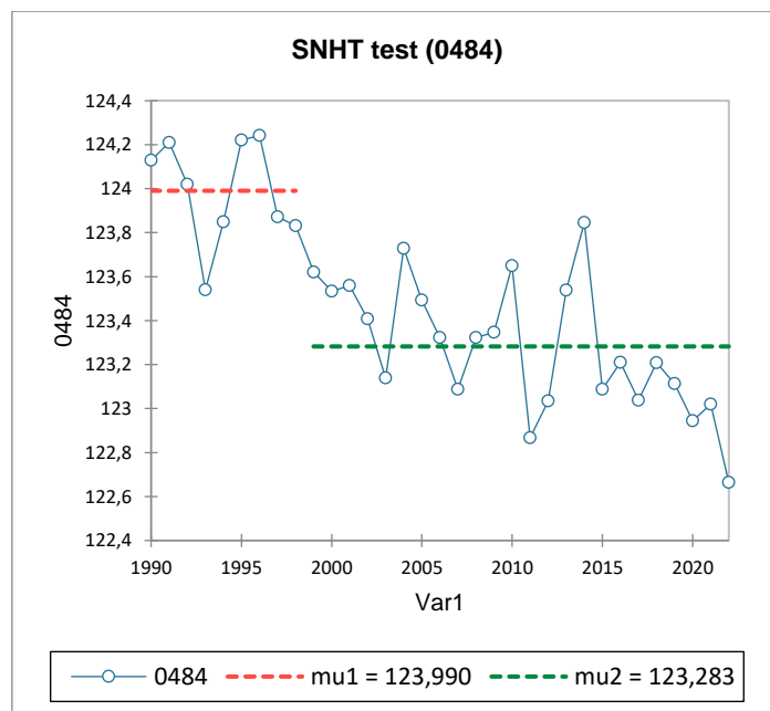
Figure 4.1.3 Example of GW lowering in the Sava river basin in Croatia
