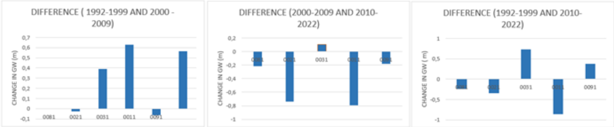
Figure 3.5.5 Differences in average GW levels between decades
