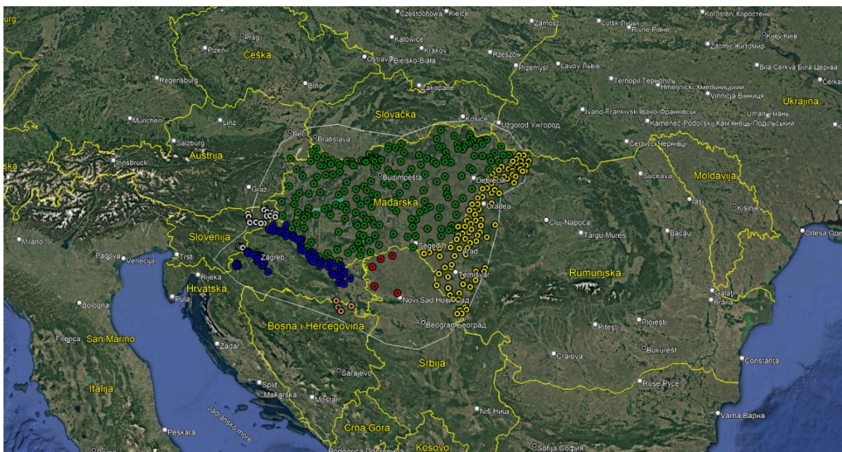
Figure 2.7.2. Presentation of reduced GW observation network ( Map 2)
