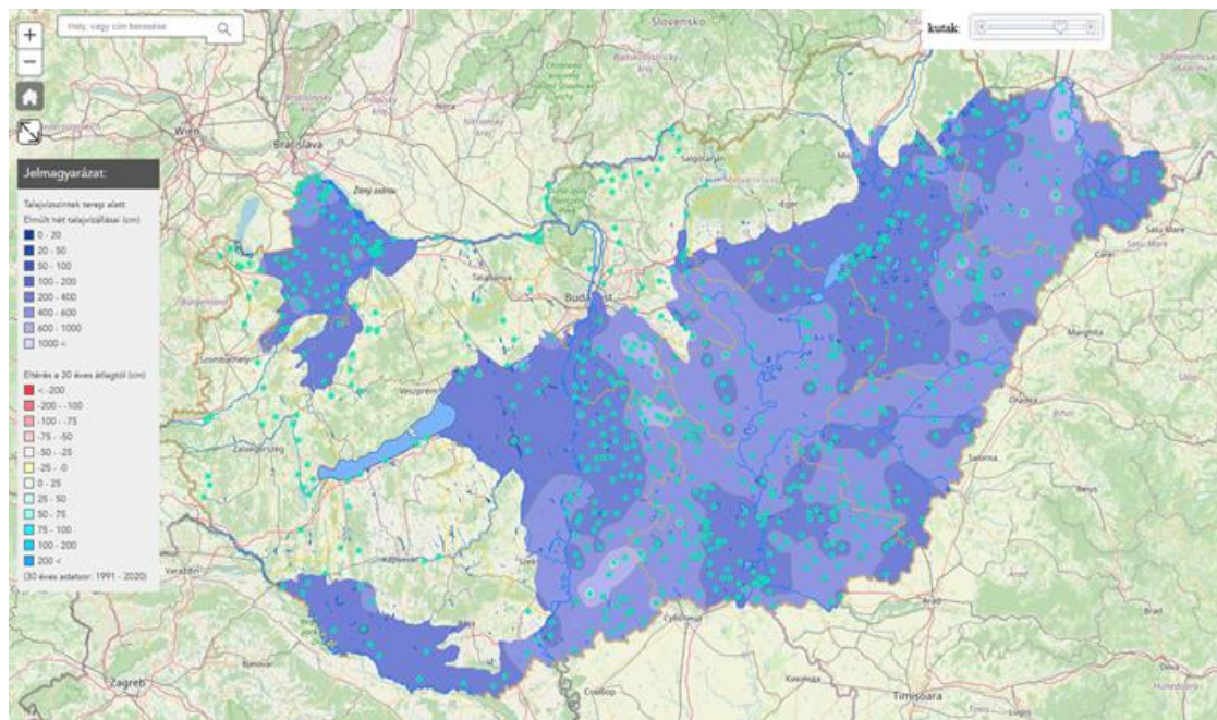
Figure 2.5.1 The network of Hungarian groundwater wells https://geoportal.vizugy.hu/talajvizkutak/index.html
