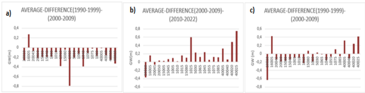
Figure 3.4.4 Differences in average GW levels between decades
