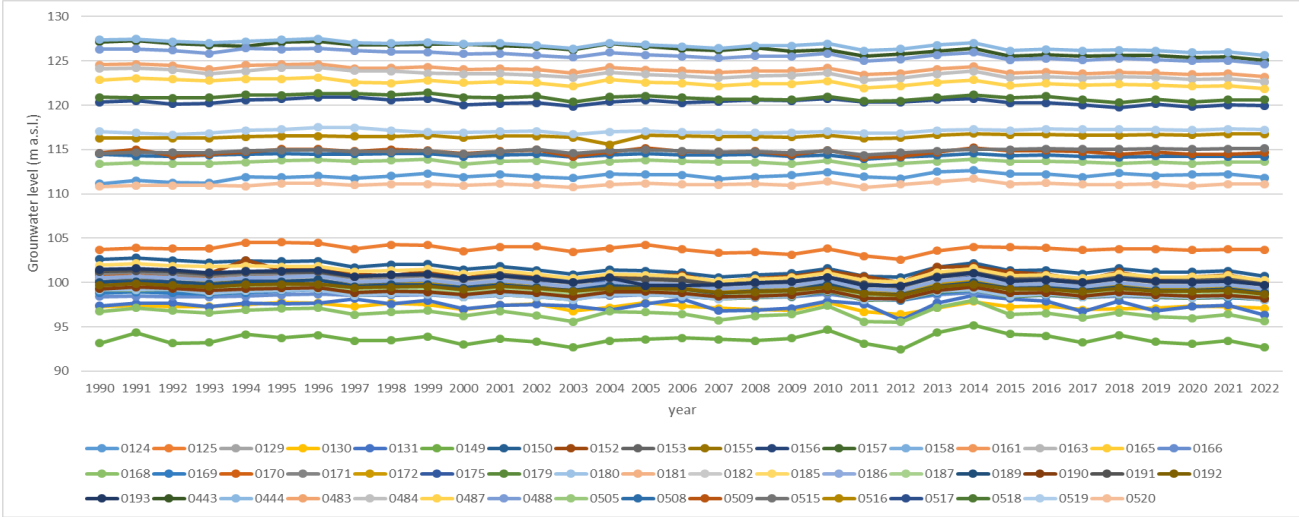
Figure 3.3.2.b) Groundwater change of obs. wells in the Sava River basin (1990-2022)
