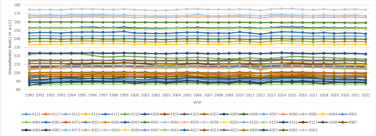
Figure 3.3.1 a) Groundwater change of obs. wells in the Drava River basin (1990-2022)
