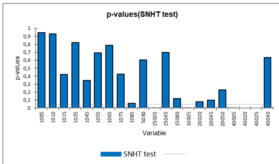
Figure 3.4.2 Results of SNHT for 21 obs. wells in Slovenia
