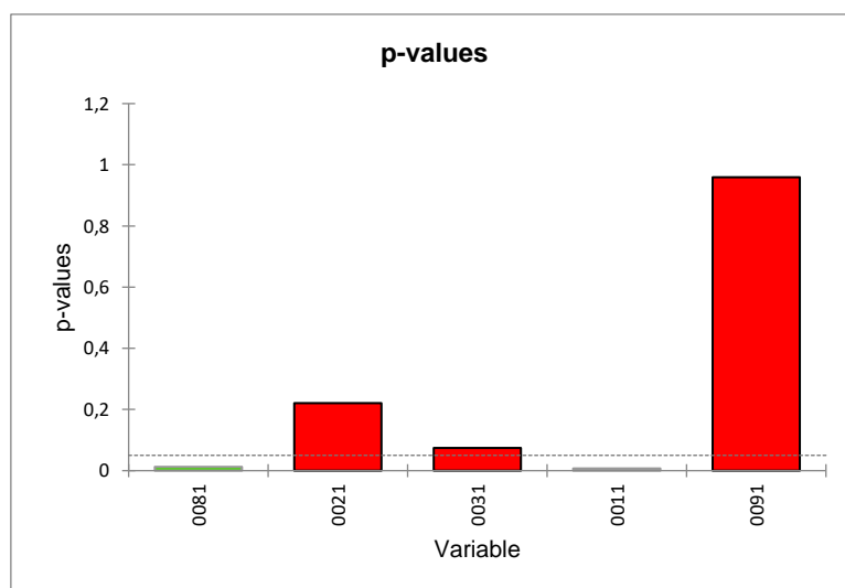
Figure 3.5.4 Results of Mann- Kendall trend test
