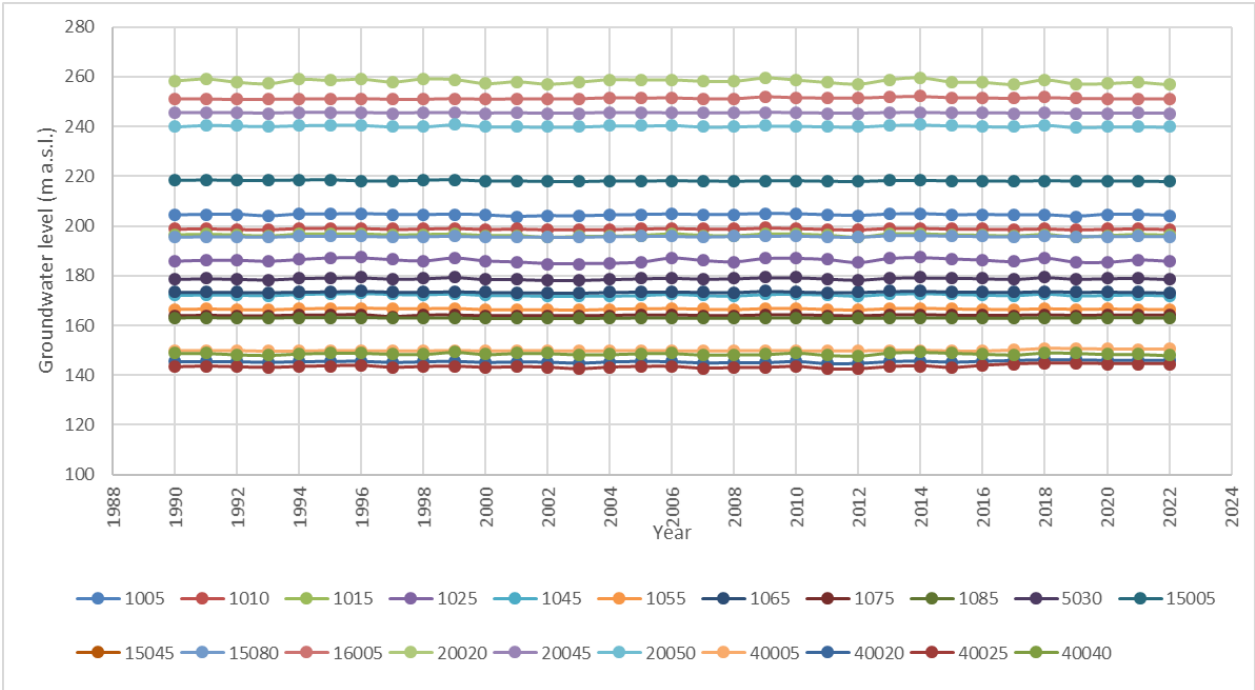
Figure 3.4.1 Groundwater change of obs. Wells in Slovenia (1990-2022)
