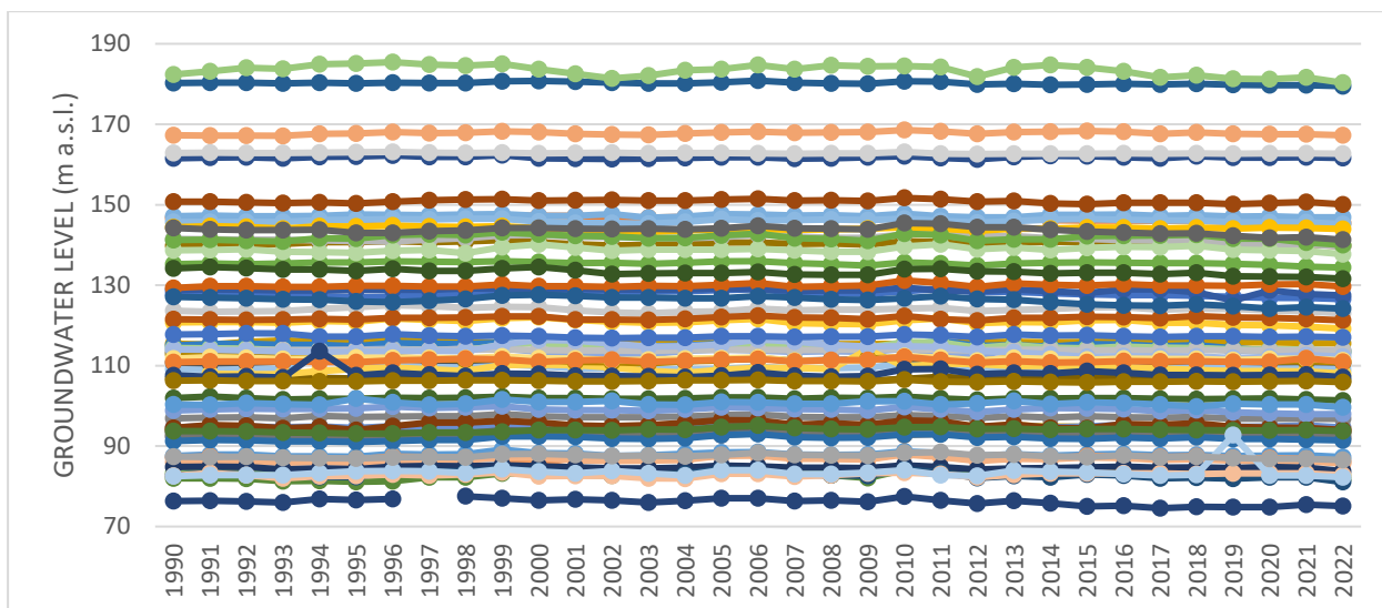
Figure 3.6.1.b) Groundwater change of 65 obs. wells in Hungary (1990-2022)
