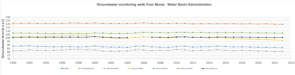
Figure 3.2.1.b) Groundwater change of obs. wells in the Mures water basin (1990-2022)
