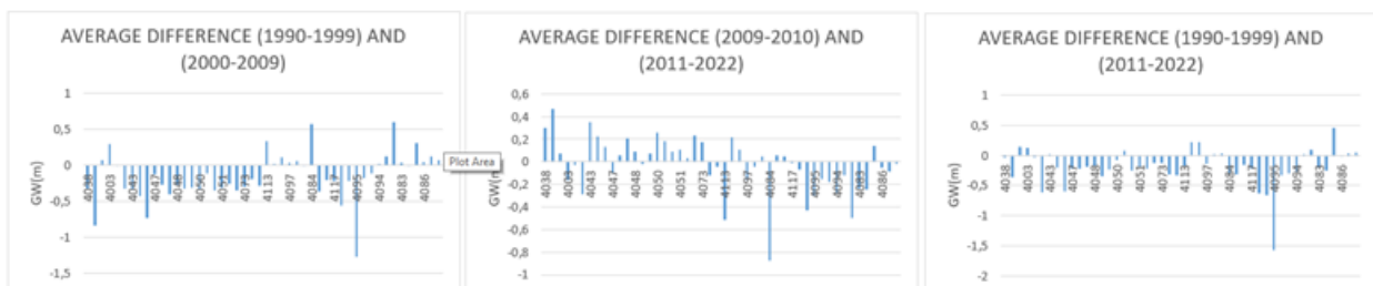
Figure 3.3.5 Differences in average annual GW levels between decades-the Drava river basin
