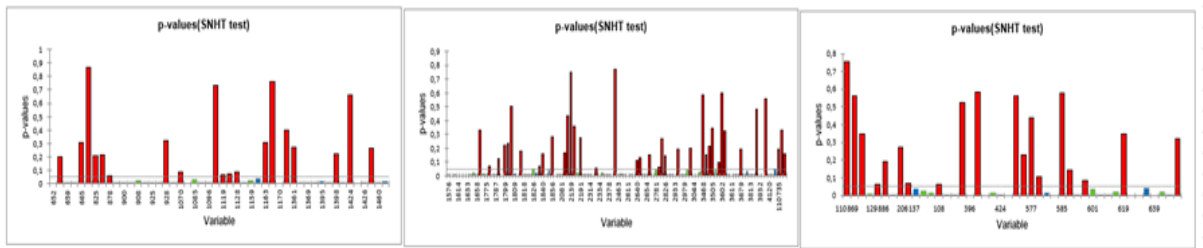
Figure 3.6.2 Results of SNHT for 200 obs. wells in Hungary divided in 3 groups
