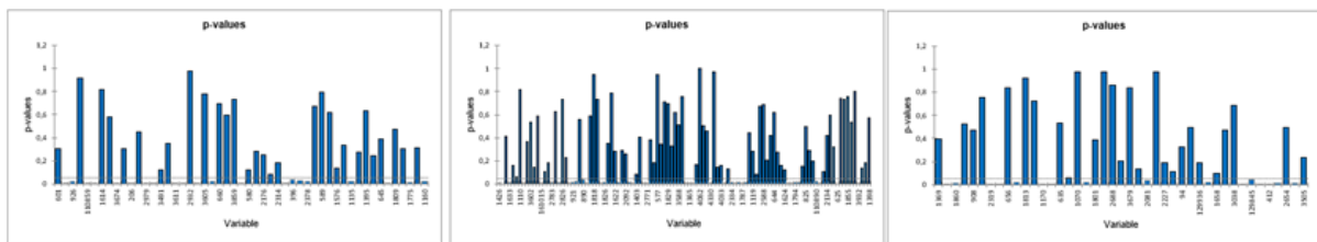
Figure 3.6.3 Results of Mann- Kendall trend test
