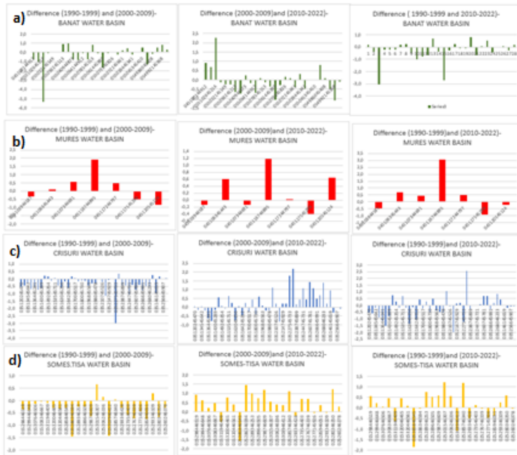
Figure 3.2.4 Differences in average GW levels for Mures, Banat, Crisuri and Somes-Tisa water basins-- Romania
