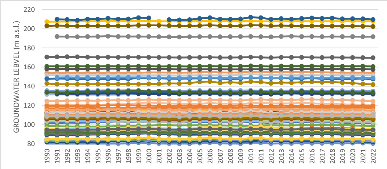
Figure 3.6.1.a) Groundwater change of 70 obs. wells in Hungary (1990-2022)
