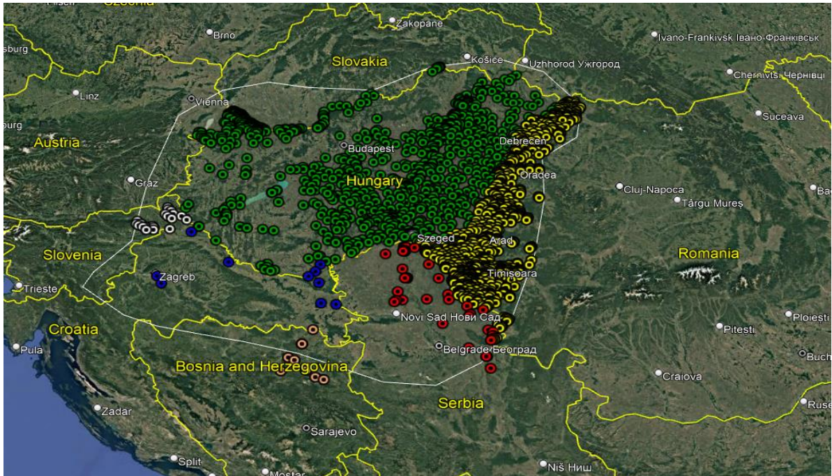
Figure 2.7.3. Map of excluded groundwater observation wells in Pannonian Plain ( Map 2 a)
